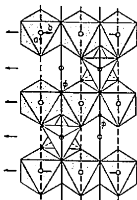
Fig. 2a. Sheet of 2[M_2O_4(TO_4)_2] showing m , \bar{1}(2) , \bar{1}(2) , 2 , 2 , and a -axial glides in space group C2/m , the ordered subgroup of P3m1 . This is the fundamental building block for the structures in the text. The axes are approximately a = 9\text{\AA} , b = 6\text{\AA} .
