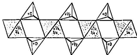
Fig. 2b. Alternative projection of 2[M_2O_4(TO_4)_2] , a frequent projection for the Fig. 5 series. The edge-sharing M\phi O_T , 6\text{\AA} octahedral chains are normal to the paper. The 9\text{\AA} direction runs from left to right and the intersheet portion runs from north to south. Heights are given as fractional coordinates of the 6\text{\AA} direction.
