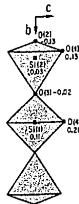
Fig. 6c. Tetrahedral interlayer link in orientite down [100]. Here, the connected [\text{Si}_3\text{O}_{10}] unit is shown.
