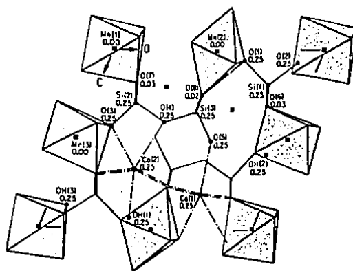
Fig. 5e. Representation of the macfallite structure down [010].
