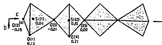
Fig. 6a. Tetrahedral interlayer link in ruizite down [100].
