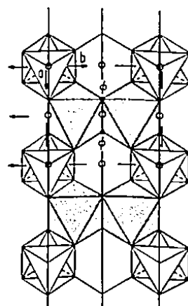
Fig. 3. The hypothetical structure built of cis\text{-}M\phi O_T octahedra. The symmetry elements m , \bar{1} are shown and the space group is P2/m . The axes are approximately a = 4.5\text{\AA} and b = 6\text{\AA} .
